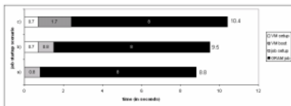
Figure 2: Xen-based VMs versus job invocation using GRAM
