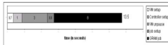
Figure 3: VM deployment time using VMware workstation
